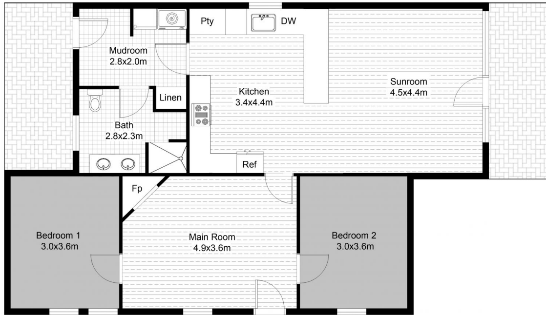
FLOOR PLAN
